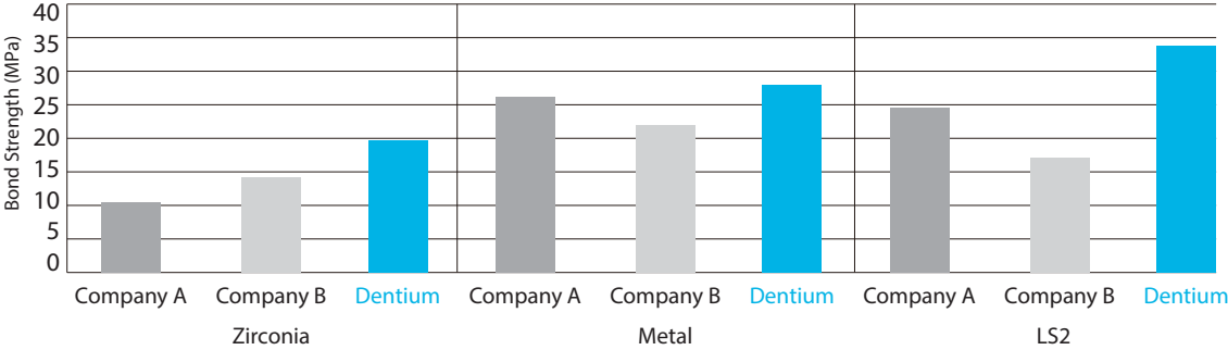
Shear bond strength to various substrates
